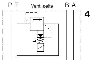
SWUVPZ-1...-T-ED-6 ... SWUVPZ-1...-T-ED-6 ...
