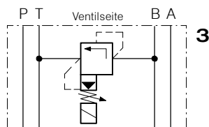
SWUVPZ-1...-BT-FA-6 ... SWUVPZ-1...-BT-FA-6 ...
