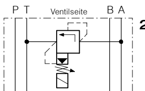
SWUVPZ-1...-AT-F-6- ... SWUVPZ-1...-AT-F-6- ...
