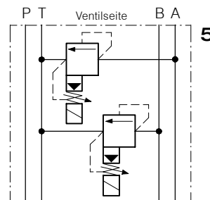
SWUVPZ-1...-ABT-J-6 ... SWUVPZ-1...-ABT-J-6 ...
